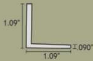
FLEXIBLE TRIM
