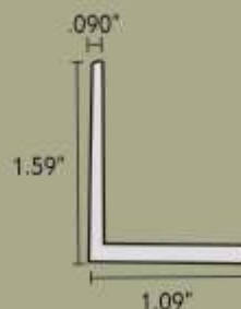
FLEXIBLE TRIM
