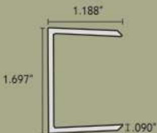
C-CHANNEL
