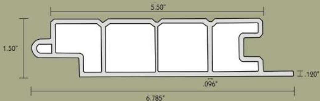
DECK BOARD
