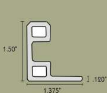
DECK STARTER
